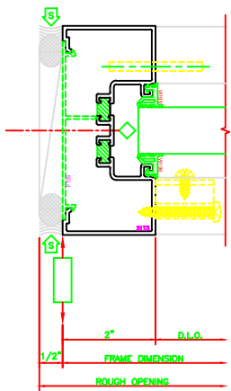
401 I.G. JAMB SERIES 403X - 2" X 4 1/2" SHEARBLOCK
