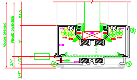
202 I.G. SILL SERIES 403X - 2" X 4 1/2" SHEARBLOCK
