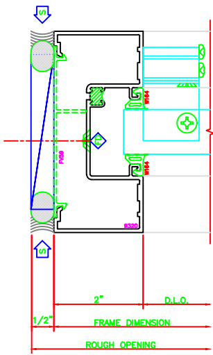
402 JAMB 403 SHEARBLOCK
