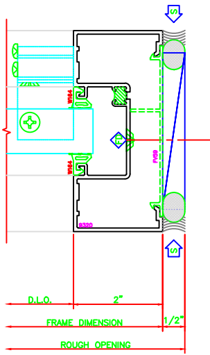
403 JAMB 403 SHEARBLOCK
