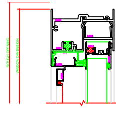
104 HEAD SERIES 3500
