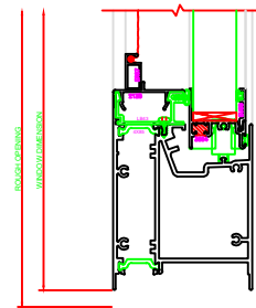
202 SILL SERIES 3500
