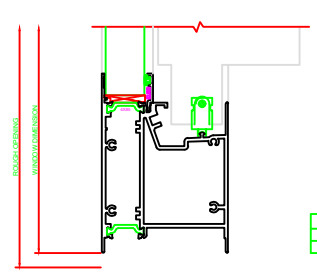
201 SILL SERIES 3500
