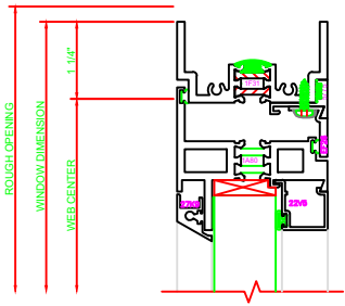
114 HEAD 550G PROJECT OUTFIXED
