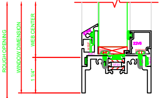
201 SILL 550G FIXED
