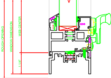
213 SILL 550G PROJECT OUTFIXED
