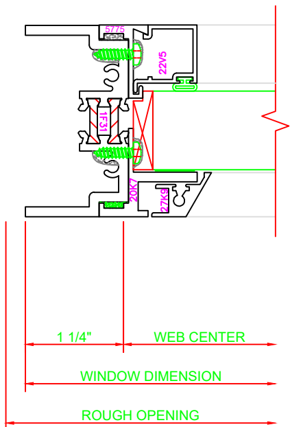
412 JAMB 550G FIXED/PROJECT IN
