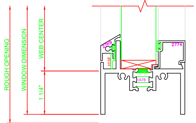
200 SILL 550G FIXED
