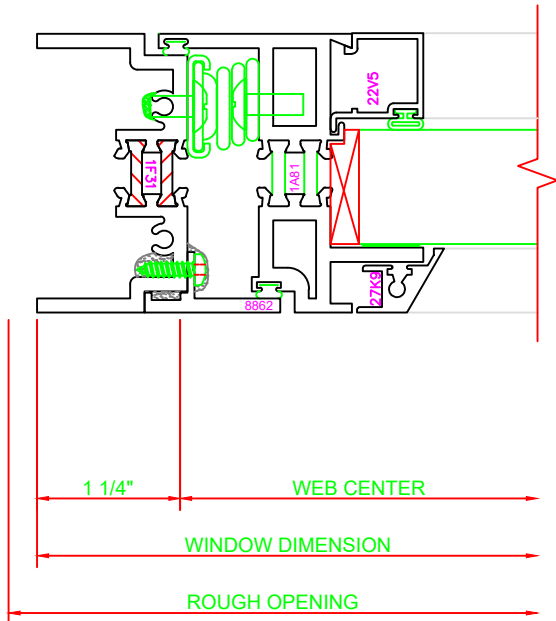
414 JAMB 550G FIXED/PROJECT IN
