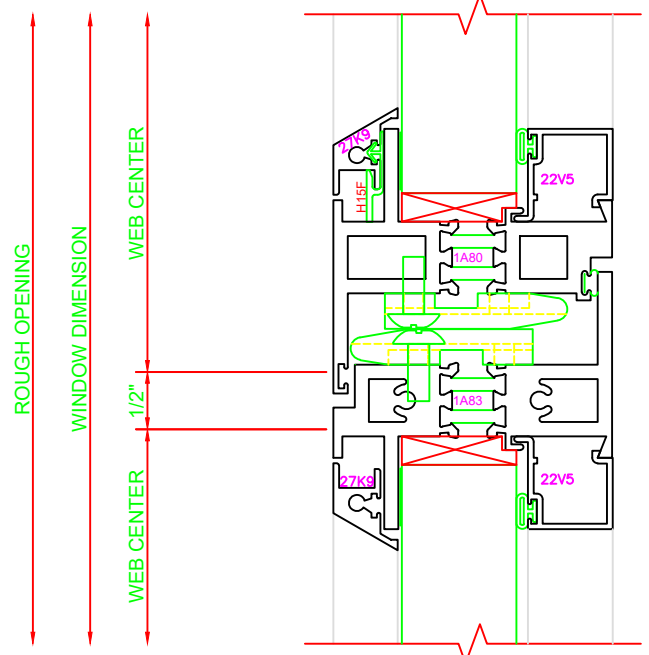
512 HORIZ. MTG. RAIL 550G CASEMENT OUT/FIXED
