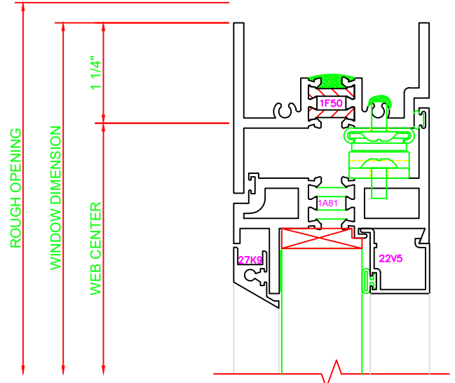
110 HEAD 550G CASEMENT IN
