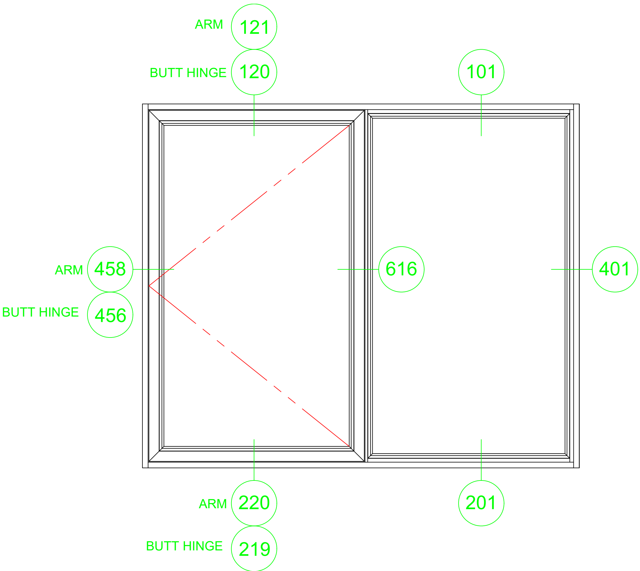
S550G INSIDE GLAZED CASEMENT OUT LEFT|FIXED BUTT HINGES AND CASEMENT ARMS
