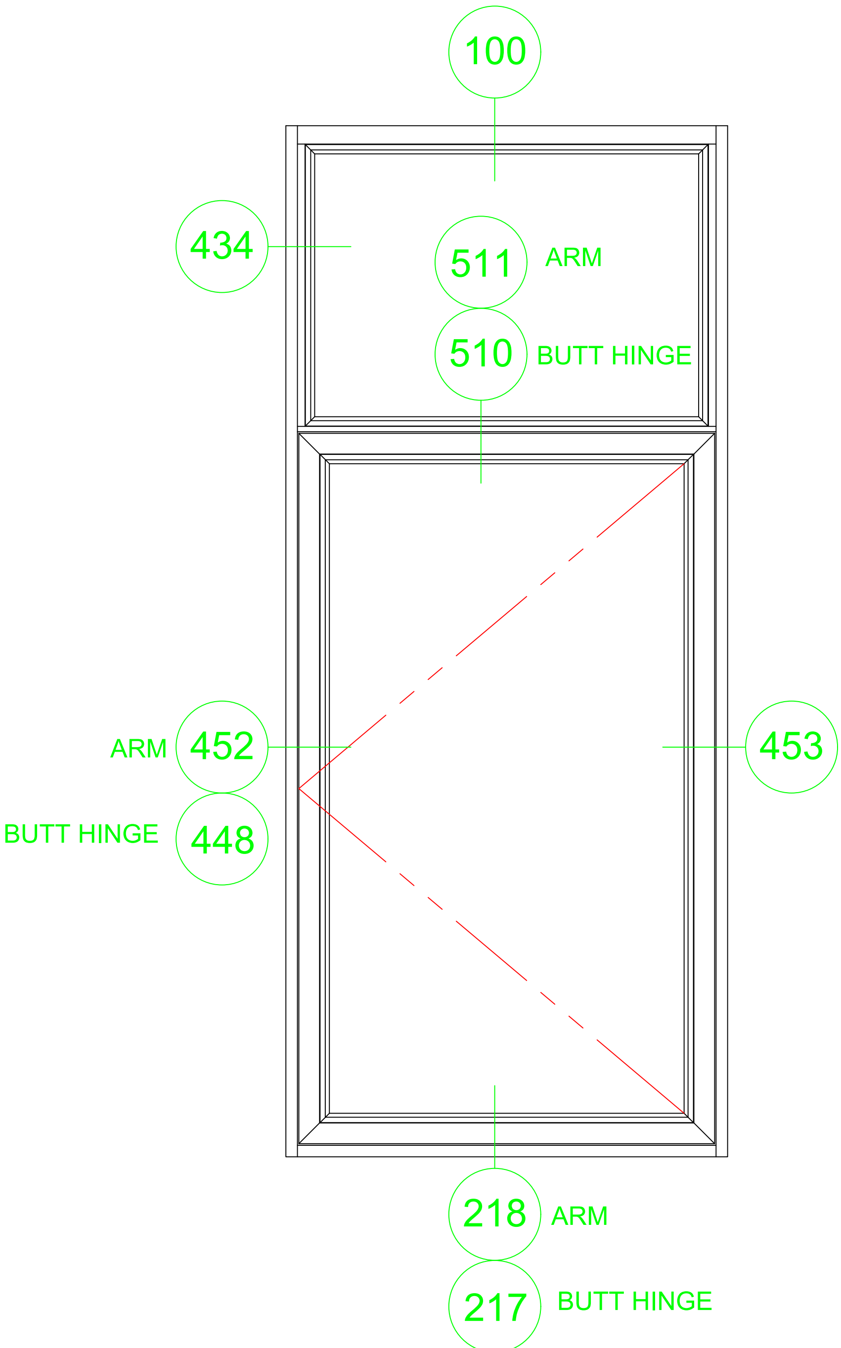
S550G INSIDE GLAZED FIXED/CASEMENT OUT LEFT BUTT HINGES AND CASEMENT ARMS
