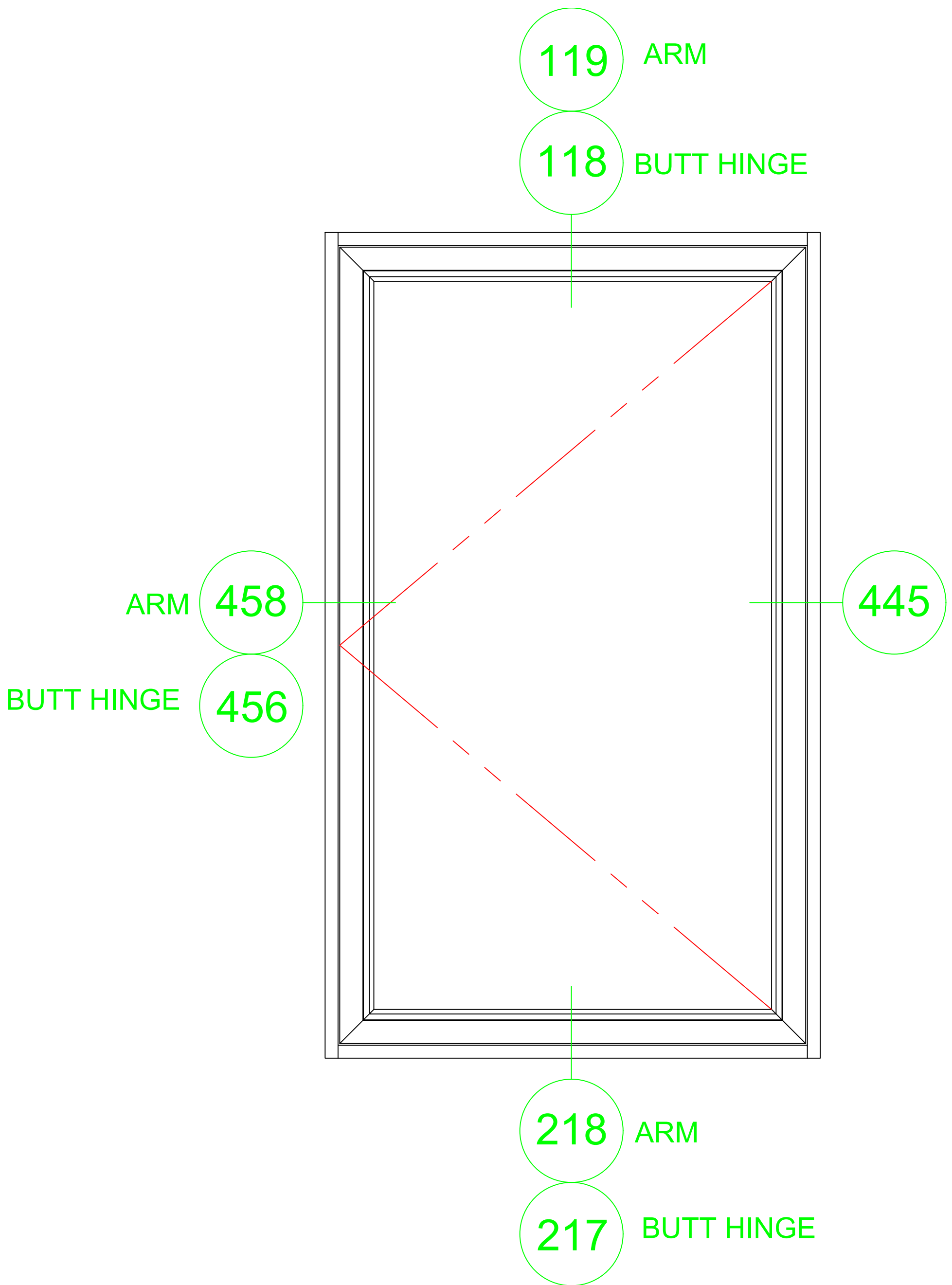
S550G INSIDE GLAZED CASEMENT OUT LEFT BUTT HINGES AND CASEMENT ARMS
