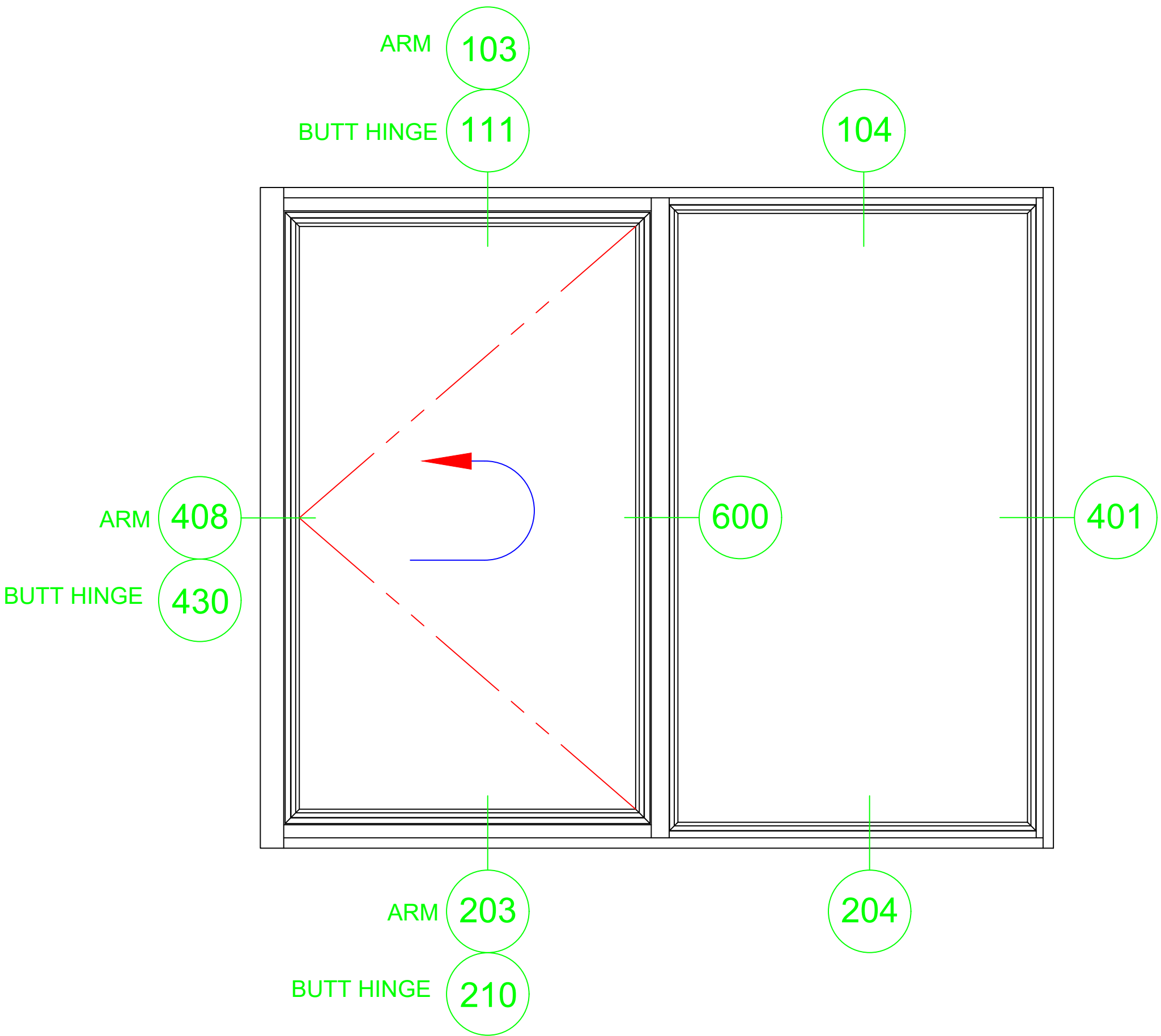
S550G INSIDE GLAZED CASEMENT IN LEFT|FIXED BUTT HINGES AND CASEMENT ARMS
