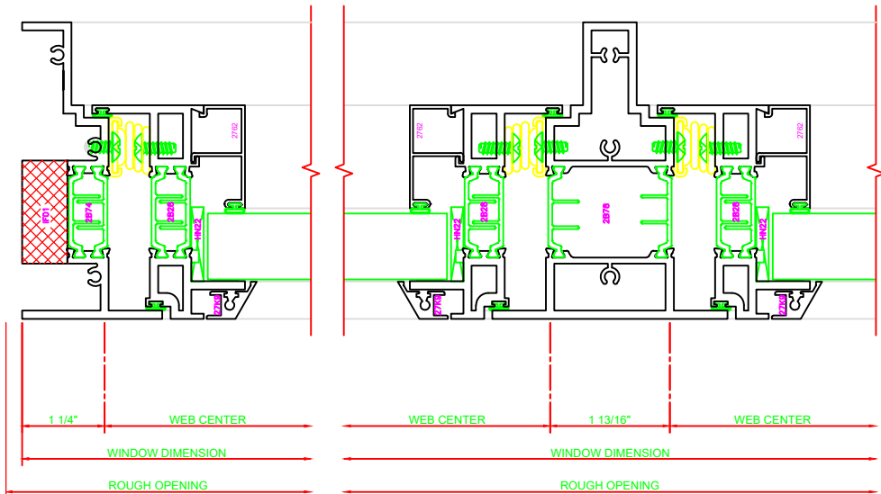
410 JAMB SERIES: 450G PROJECT IN 4-BAR ARMS
