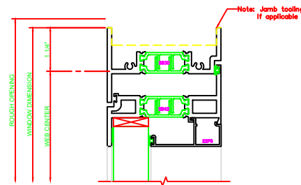
131 HEAD 325 CASEMENT IN BUTT HINGES
