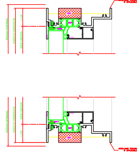
102 HEAD SERIES: 450X FIXED
