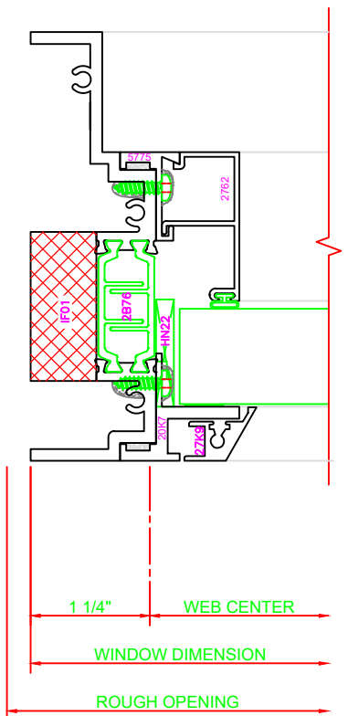
402 JAMB SERIES: 450G FIXED
