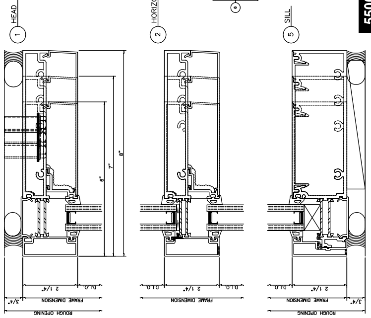
5500 Outside Glazed 2 1/4" x 6", 7", 8"
